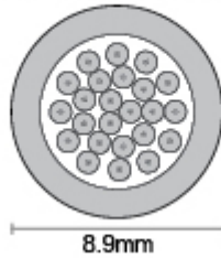
24 Fibre Tight Buffered
